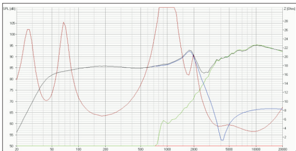
Summed frequency response at standard speaker 0 dB = 2,83V 160 mm woofer (80hm) Re: 6,2Ω Le: 1,2 mH 25 mm tweeter (80hm) Re: 6,2Ω Le: 0,1 mH
