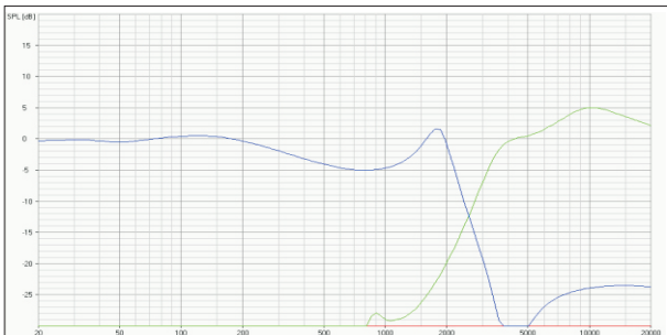
Net gain at standard speaker 0 dB = 2,83V 160 mm woofer (80hm) Re: 6,2Ω Le: 1,2 mH 25 mm tweeter (80hm) Re: 6,2Ω Le: 0,1 mH
